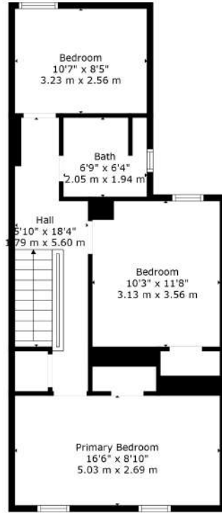
Floor 2
