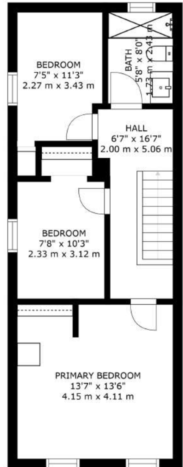
FLOOR 3
