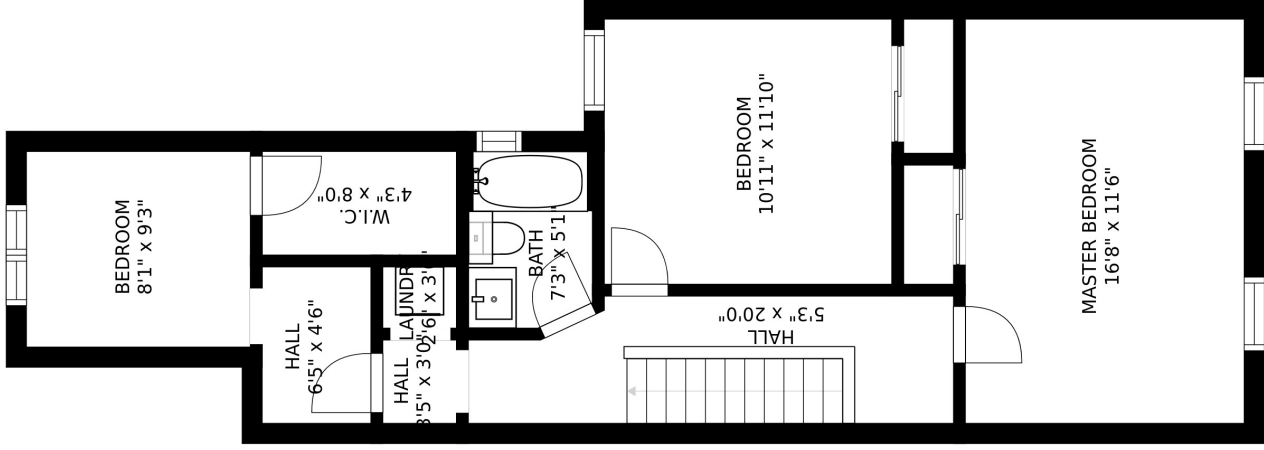
FLOOR 2
