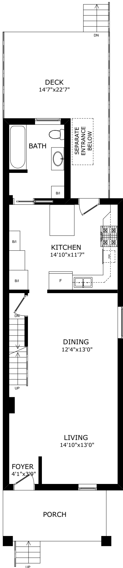
MAIN FLOOR
