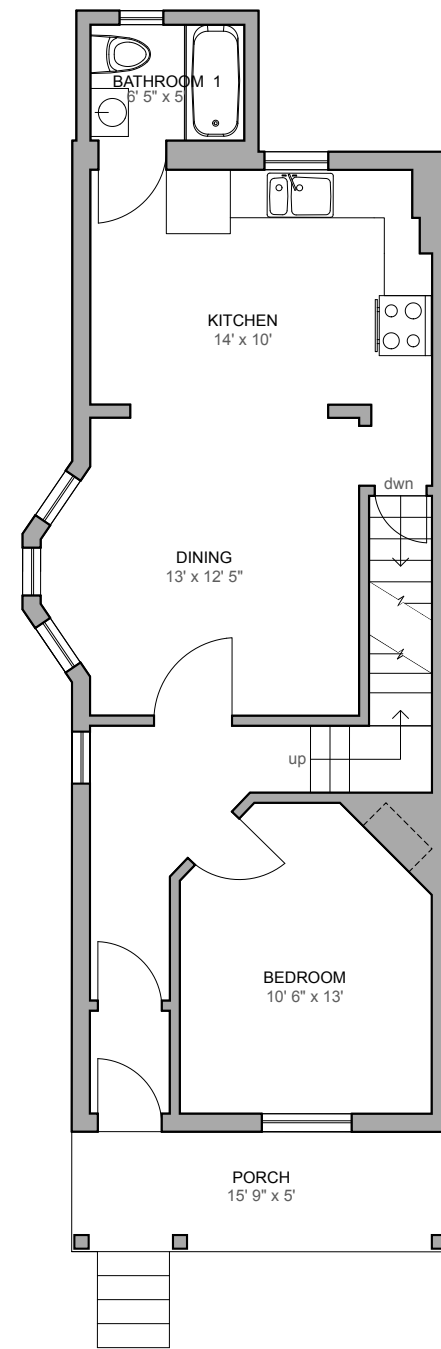
FIRST FLOOR 700 sqft
